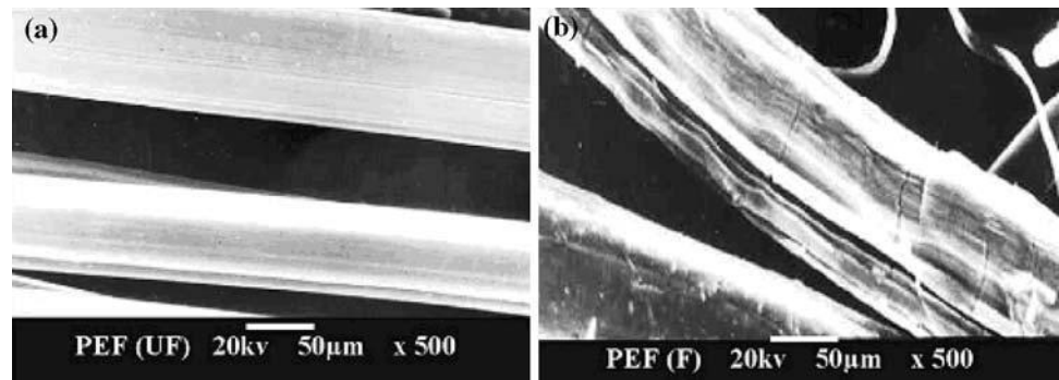
Fig. 2 SEM micrographs of a unmodified and b modified UHMWPE fibers. Source: Used with permission [92]
