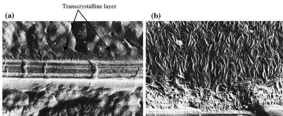
Fig. 1 Low voltage SEM images of a UHMWPE fiber/ HDPE composite showing the presence of a transcrystalline layer and b a close-up of the transcrystalline layer illustrating the presence of lamellae twisting. Source: Used with permission [50]
